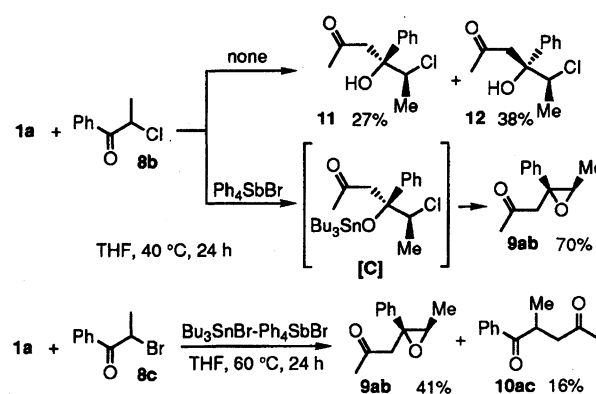
Scheme 7.
