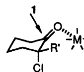
Scheme 5.
